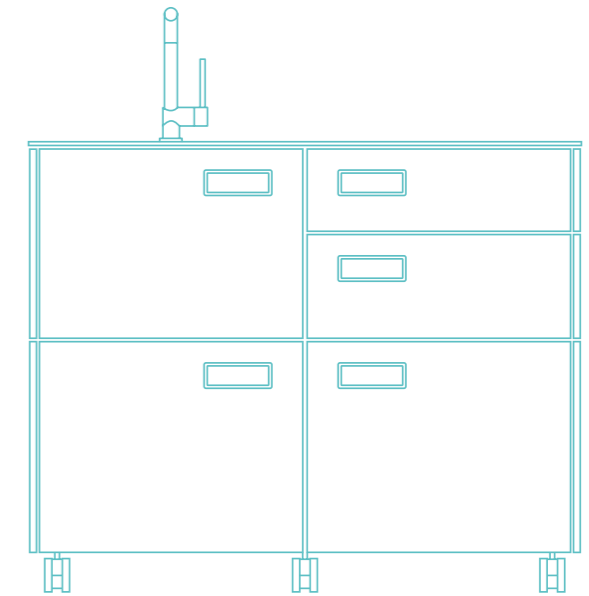
Tidy Prime Cuisine 1234 × 1012 × 605 mm
