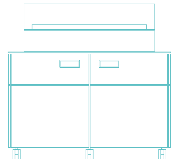
Grill Prime 1234 × 1012 × 605 mm
